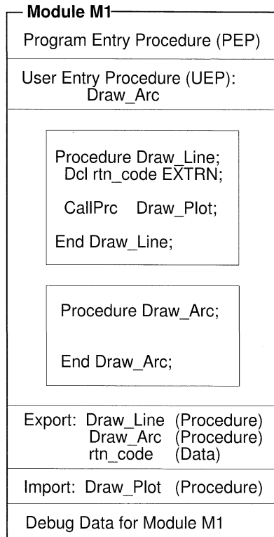
Figure 2-2. Conceptual View of a Module
